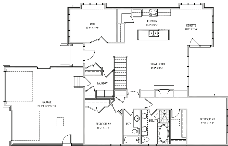
1 MAIN FLOOR PLAN - 1685 SQ FT
