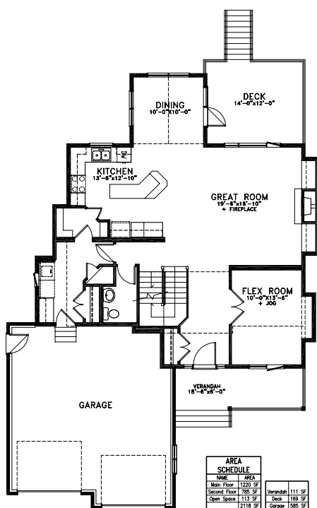
MAIN FLOOR PLAN NTS
