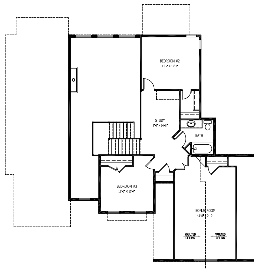
2 SECOND FLOOR PLAN - 961 SQ FT 1/8" = 1'-0"
